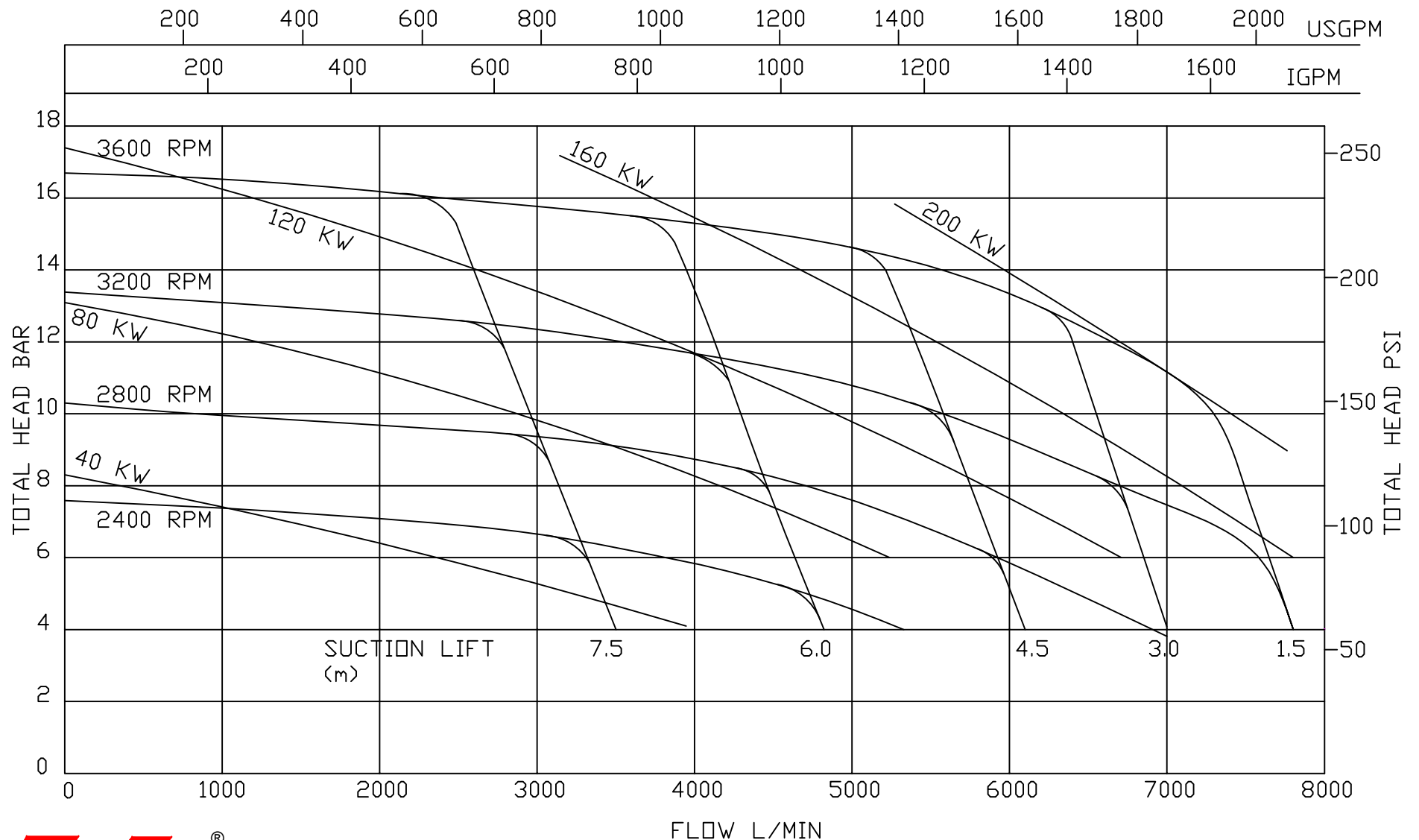
TYPICAL PERFORMANCE CURVE OF MFV LP 1060
